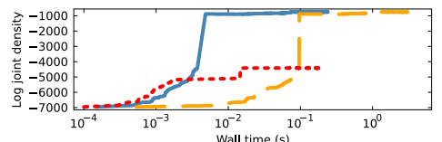
(g) Wrong inference result by Gen due to an incrementalization bug (on a binary mixture model).
